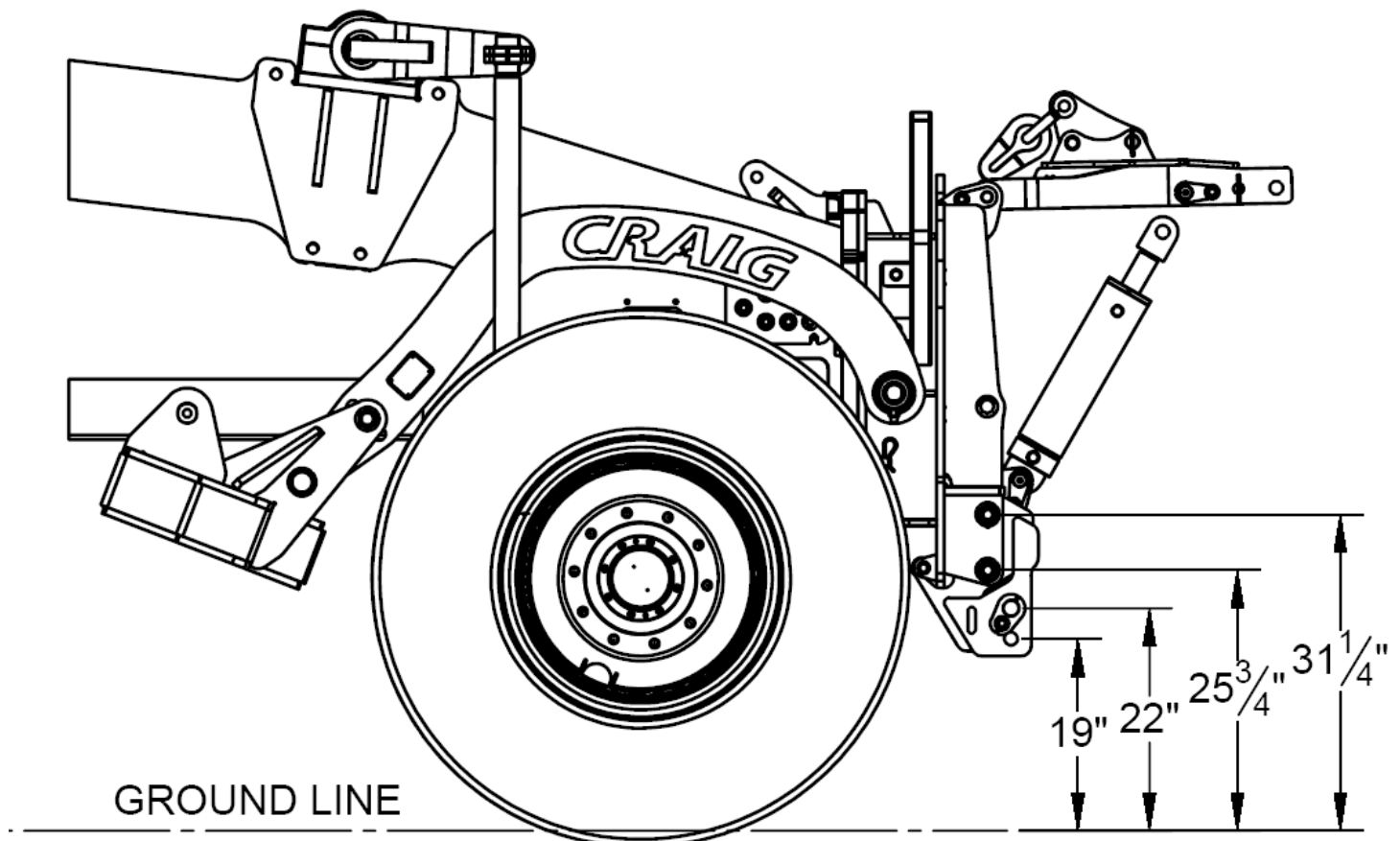
HEIGHTS OF PIN HOLES
