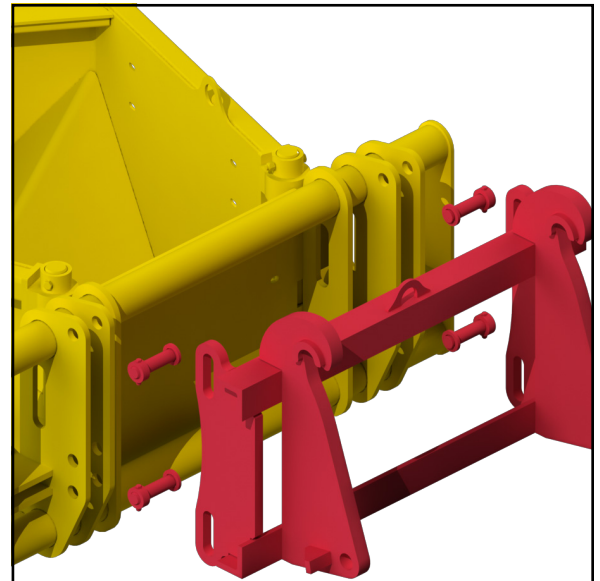
Modular hook-up with built in float.
